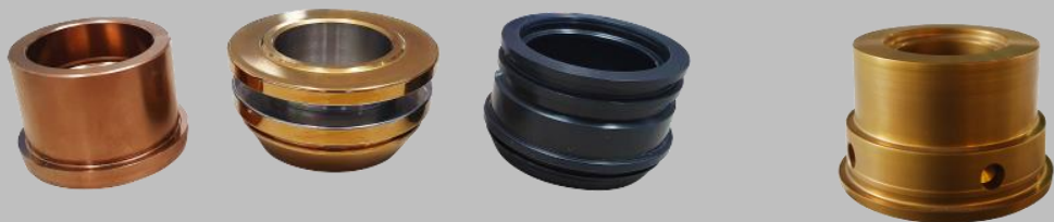
Seaming Tools: Stellite, 1.2379, 1.4528 Coatings CVD-TiN, TiC, TiCN, Al 2 O 3
